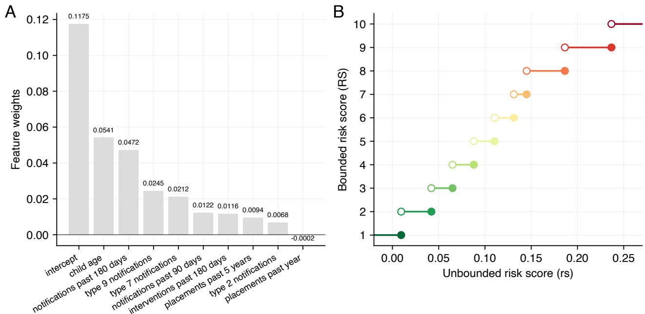
Figure 2: The Decision Support (DSS) model. A, Feature weights of the model, sorted according to magnitude. The weight for x_{placements\ past\ year} is too small to be visually observed. B, Bounds used to transform unbounded risk scores ( rs ) to bounded risk scores ( RS ). Open circles indicate half-open intervals.
