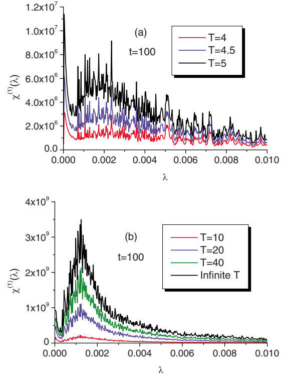
FIG. 4. (Color online) The first term of the OFS, \chi^{(1)}(\lambda) , with K=120 , D_c=800 , and t=100 for (a) small temperatures and (b) higher temperatures. Notice that \chi^{(1)} grows with temperature.
