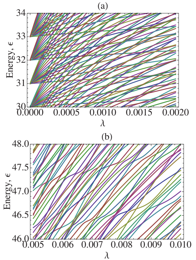
FIG. 2. (Color online) Eigenenergies vs coupling strengths for K=120 for (a) couplings 0 < \lambda < 2 \times 10^{-3} and energies 30 < E < 34 , such that 0 < \eta < 2.3 , and (b) couplings 5 \times 10^{-3} < \lambda < 10^{-2} , such that 10 < \eta < 23 .
