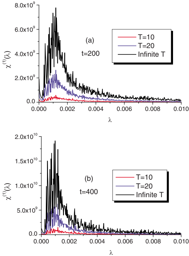
FIG. 5. (Color online) The first term of the OFS, \chi^{(1)}(\lambda) , with K=120 , D_c=800 , and various high temperatures at (a) t=200 (b) t=400 . Again, observe that \chi^{(1)} grows with temperature.
