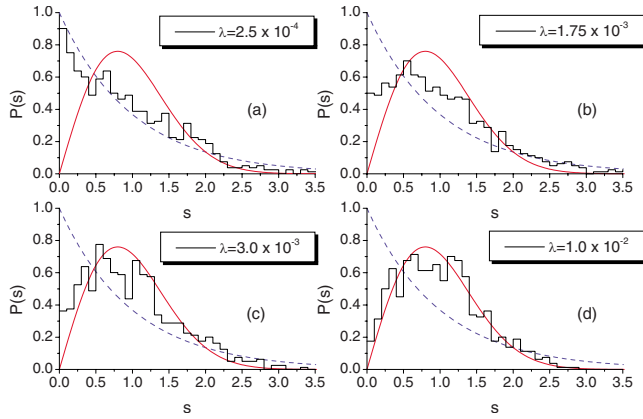
FIG. 1. (Color online) Level spacing distributions for (a) \lambda = 2.5 \times 10^{-4} , approximately the location of the local minimum of \chi^{(1)}(\lambda) , (b) \lambda = 1.75 \times 10^{-3} , approximately the peak of \chi^{(1)}(\lambda) , (c) \lambda = 3.0 \times 10^{-3} , in the tail of the peak, and (d) \lambda = 1.0 \times 10^{-2} , far into the quantum chaotic regime. Here all 800 well-converged levels are included in the statistics. The Poisson statistics are given by P(s) = e^{-s} (dashed curve) and the Wigner-Dyson statistics are P(s) = \frac{\pi}{2} s e^{-(\pi/4)s^2} (solid curve).
