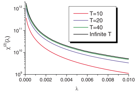
FIG. 6. (Color online) The second term of the OFS, \chi^{(2)}(\lambda) , taking K=120 , D_c=800 , and t=100 . Note that this quantity increases with temperature.
