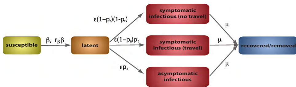
Fig. 3. Compartmental structure of the epidemic model within each subpopulation. A susceptible individual in contact with a symptomatic or asymptomatic infectious person contracts the infection at rate \beta or r_\beta \beta , respectively, and enters the latent compartment where he is infected but not yet infectious. At the end of the latency period \varepsilon^{-1} , each latent individual becomes infectious, entering the symptomatic compartments with probability 1 - p_a or becoming asymptomatic with probability p_a . The symptomatic cases are further divided between those who are allowed to travel (with probability p_t ) and those who would stop traveling when ill (with probability 1 - p_t ). Infectious individuals recover permanently with rate \mu . All transition processes are modeled through multinomial processes.
